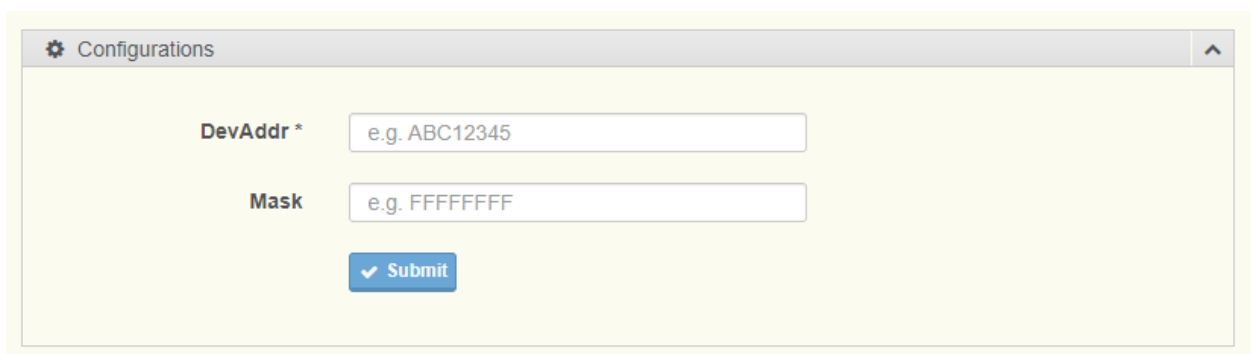
Figure 2.26 Create Ignored
