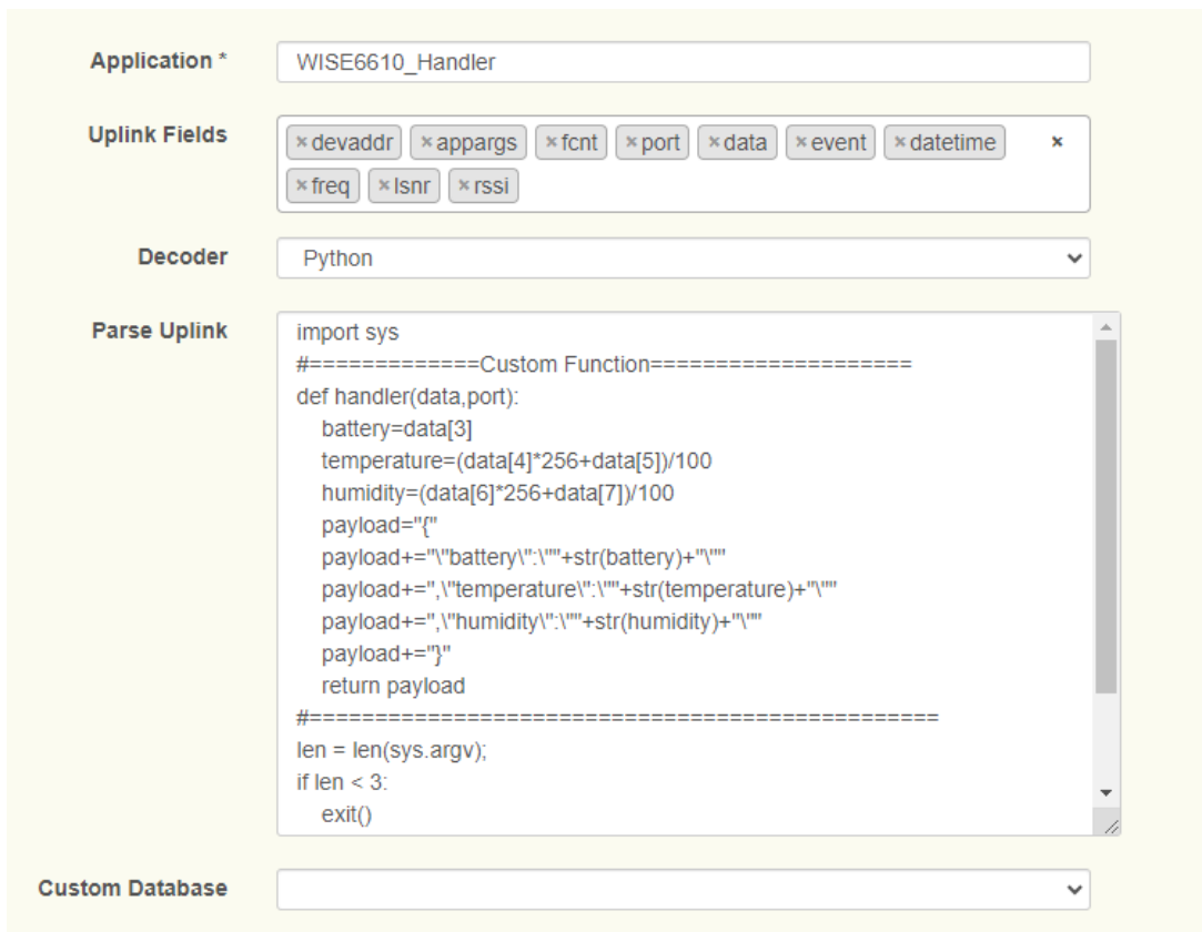
Figure 2.42 Handler using Python
